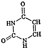
Uracil (2,6-dioxy-pyrimidine)
