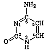
Cytosine (2-oxy-6-aminopyrimidine)
