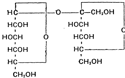
Sucrose
