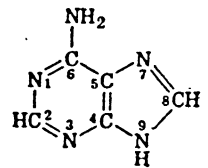
Adenine (6-aminopurine)
