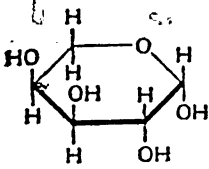
\beta -L-Arabinopyranose
