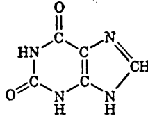
Xanthine (2,6-dioxypurine)
