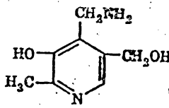
Pyridoxamine
