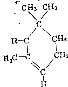
( \alpha -Ionone)
