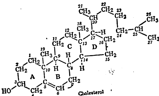
Cholesterol ( C_{27}H_{45}OH )
