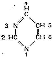
Pyrimidine
