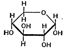
\alpha -D-Xylopyranose
