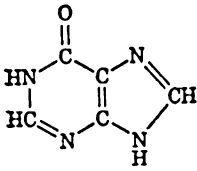
Hypoxanthine (6-oxypurine)
